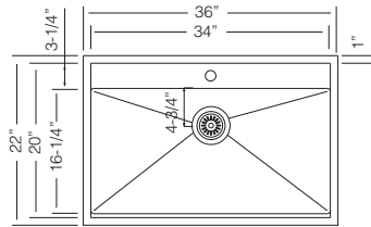
GRS 914 St.Steel Grid
